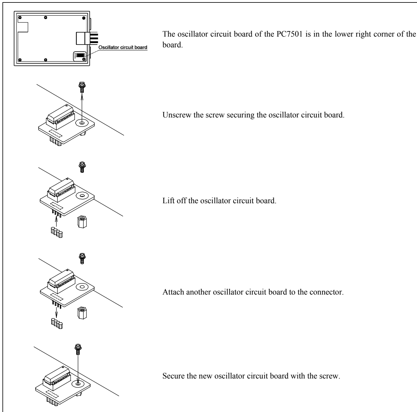
Figure 2.18 Replacing oscillator circuit boards
